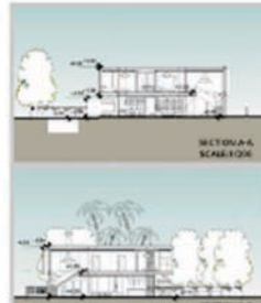
SECTION A SCALE 1:100
